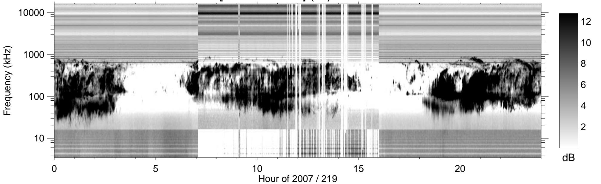
RPWS [ABCH1H2/Ex] (-B) 2007/08/07
