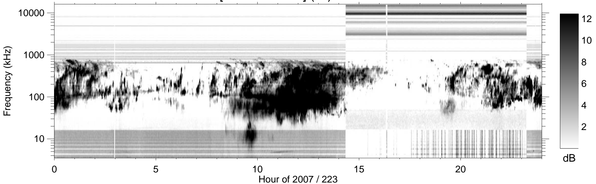
RPWS [ABCH1H2/Ex] (-B) 2007/08/11
