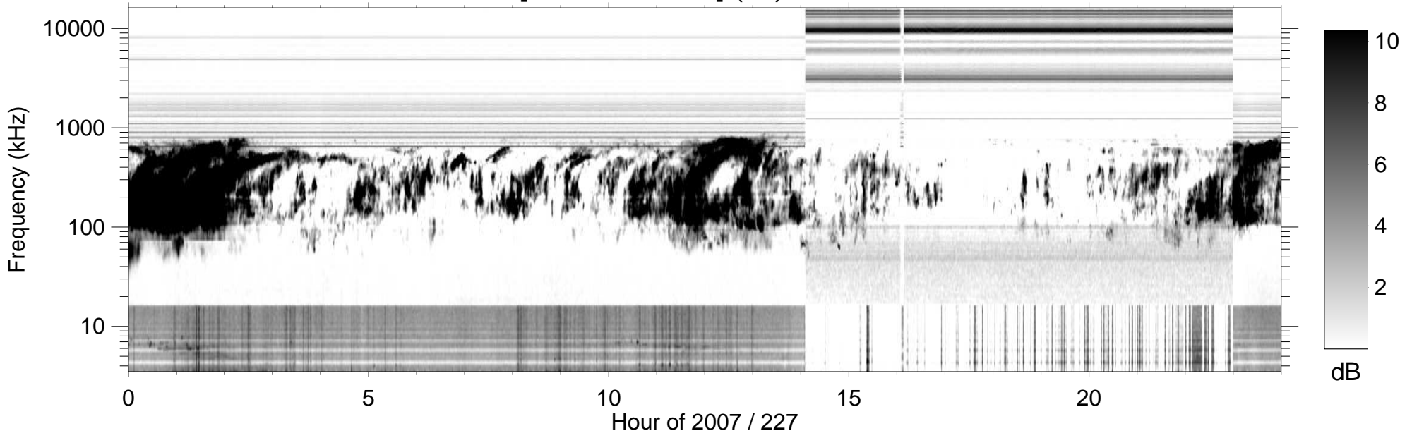
RPWS [ABCH1H2/Ex] (-B) 2007/08/15
