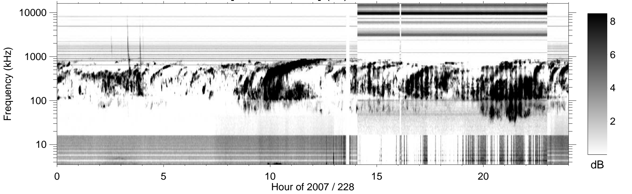
RPWS [ABCH1H2/Ex] (-B) 2007/08/16
