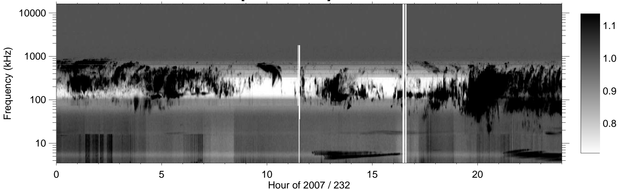
RPWS [ABCH1H2/Ex] (-B) 2007/08/20
