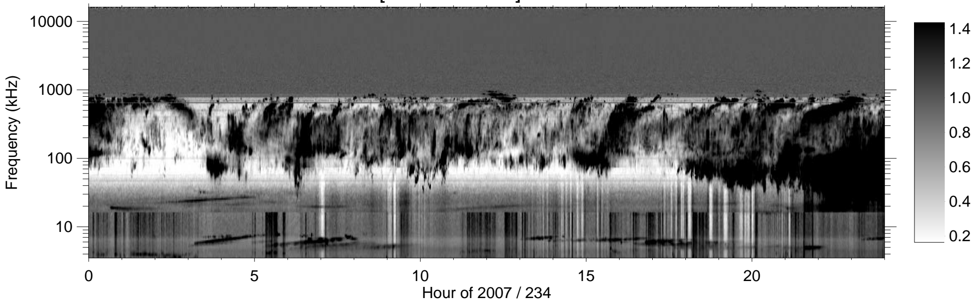
RPWS [ABCH1H2/Ex] (-B) 2007/08/22
