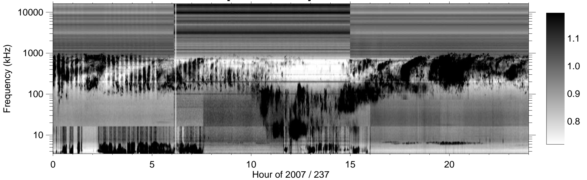
RPWS [ABCH1H2/Ex] (-B) 2007/08/25
