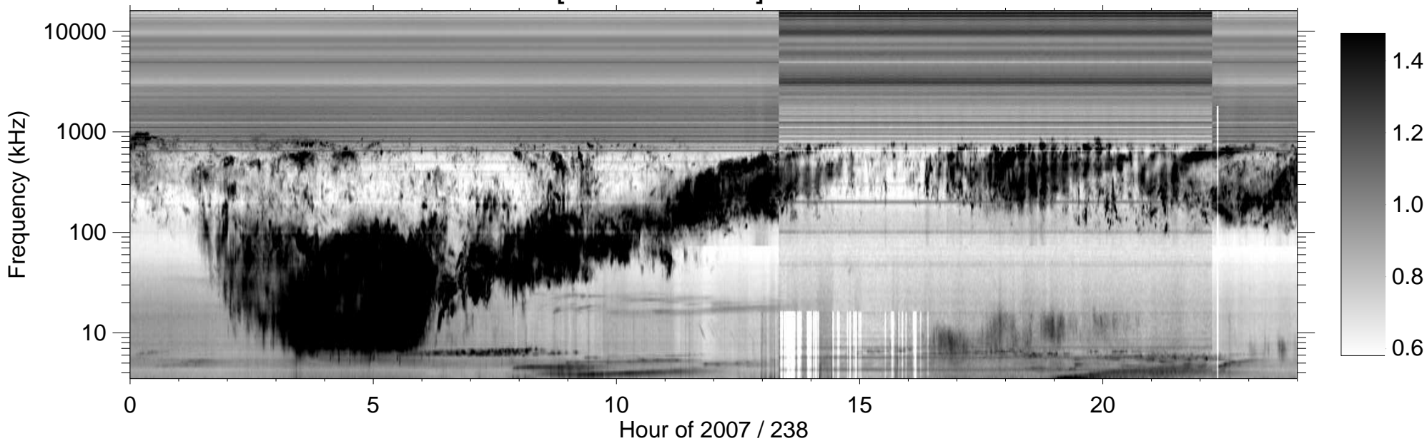
RPWS [ABCH1H2/Ex] (-B) 2007/08/26
