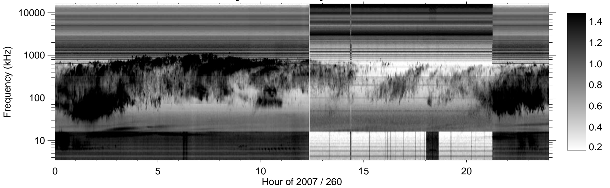
RPWS [ABCH1H2/Ex] (-B) 2007/09/17
