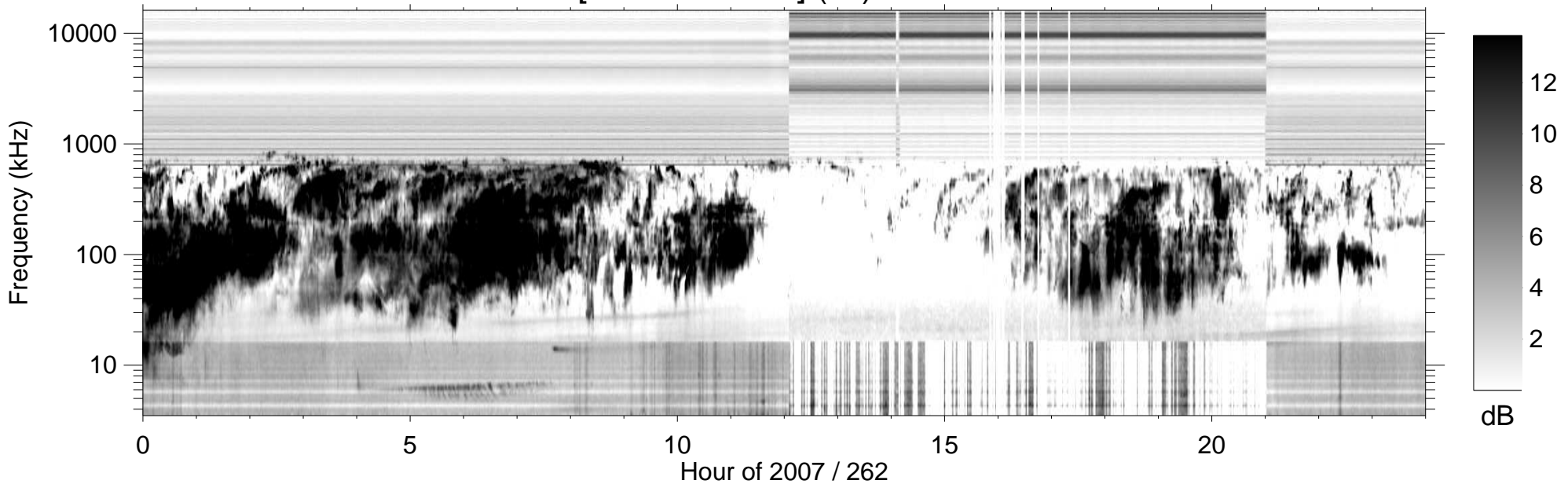
RPWS [ABCH1H2/Ex] (-B) 2007/09/19
