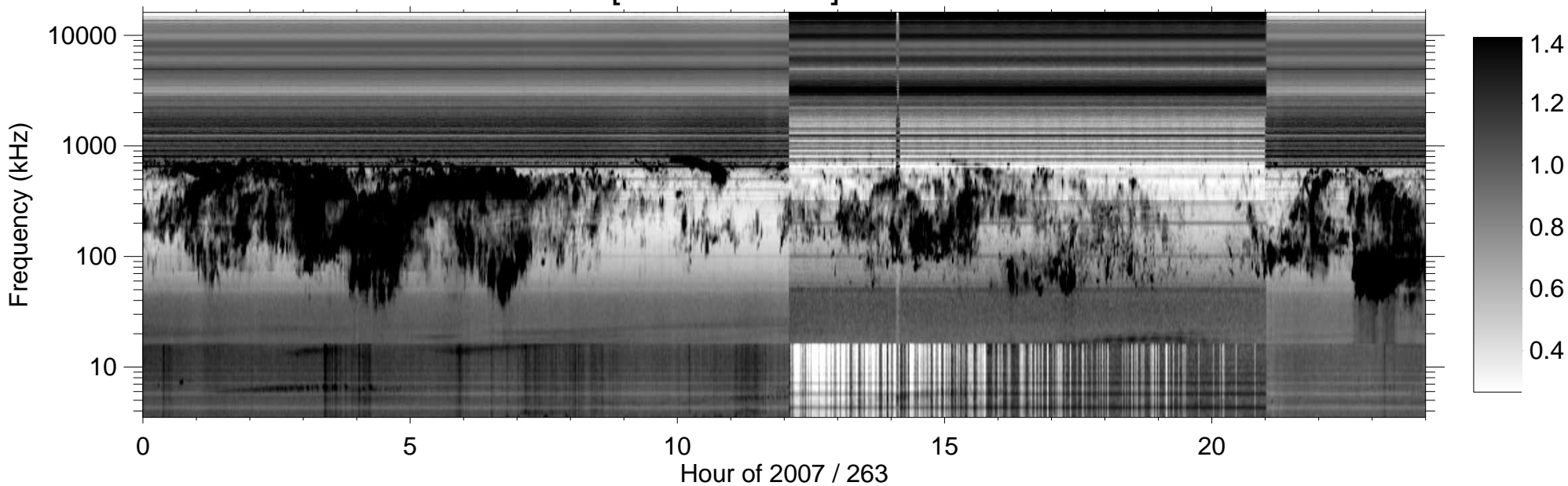
RPWS [ABCH1H2/Ex] (-B) 2007/09/20
