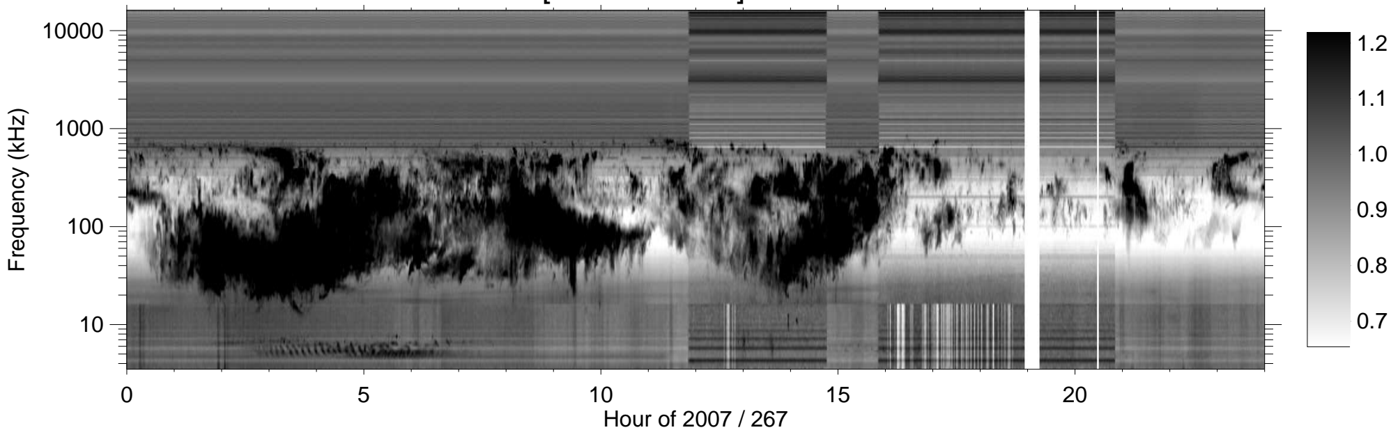
RPWS [ABCH1H2/Ex] (-B) 2007/09/24
