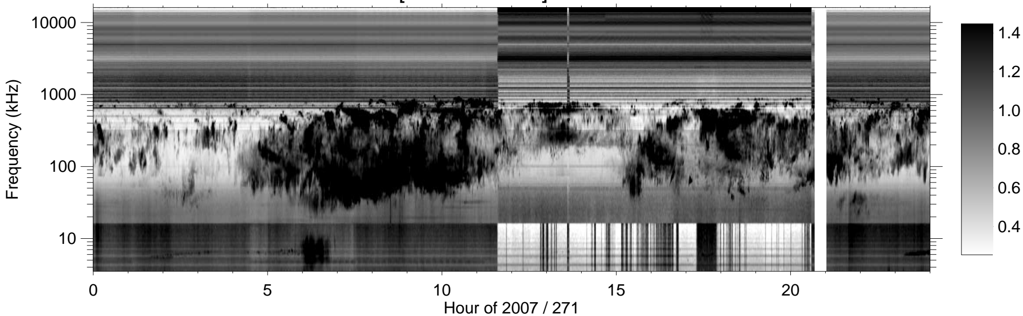
RPWS [ABCH1H2/Ex] (-B) 2007/09/28
