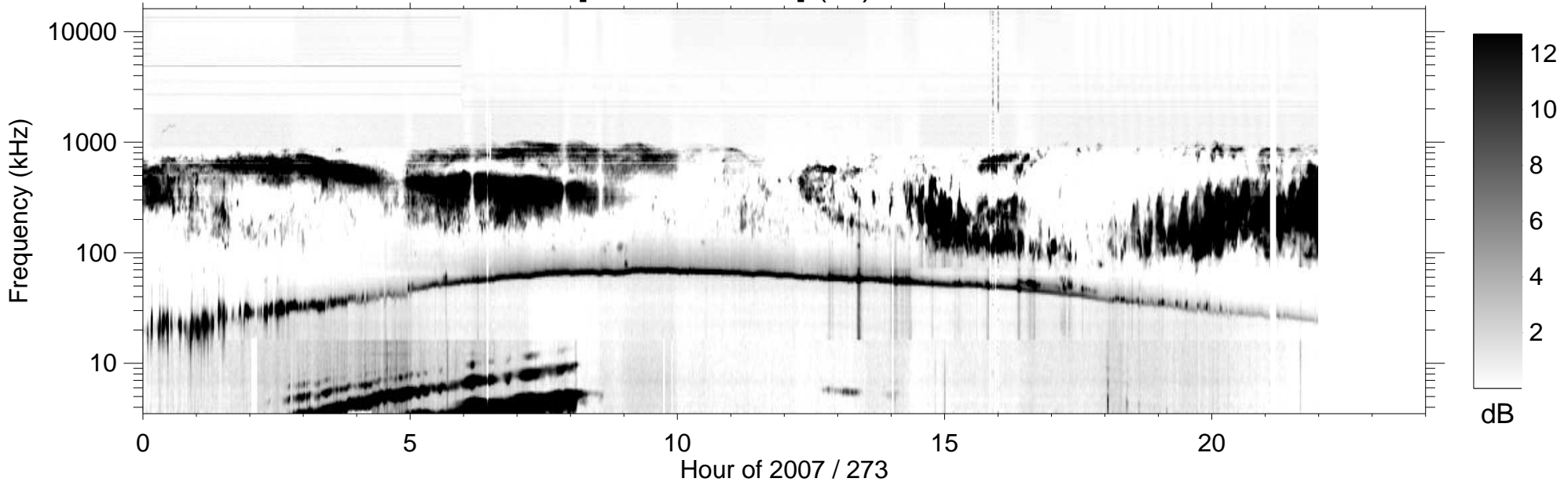
RPWS [ABCH1H2/Ex] (-B) 2007/09/30
