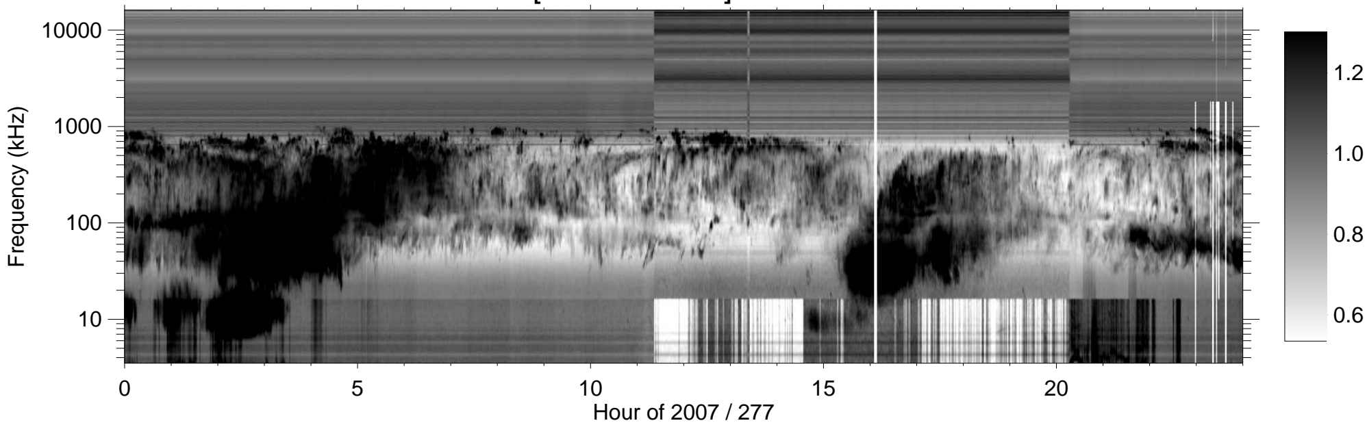
RPWS [ABCH1H2/Ex] (-B) 2007/10/04
