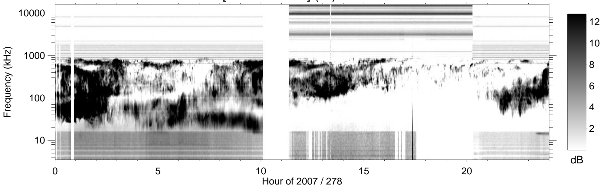
RPWS [ABCH1H2/Ex] (-B) 2007/10/05
