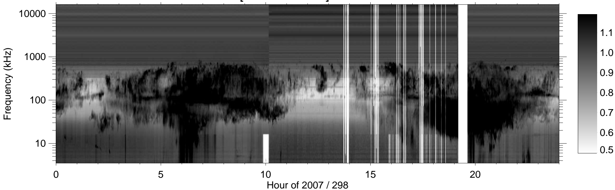
RPWS [ABCH1H2/Ex] (-B) 2007/10/25
