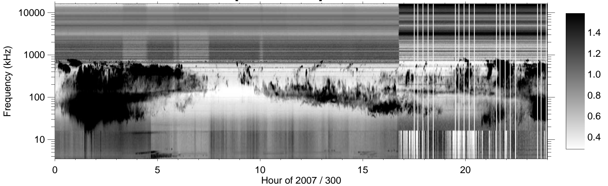
RPWS [ABCH1H2/Ex] (-B) 2007/10/27
