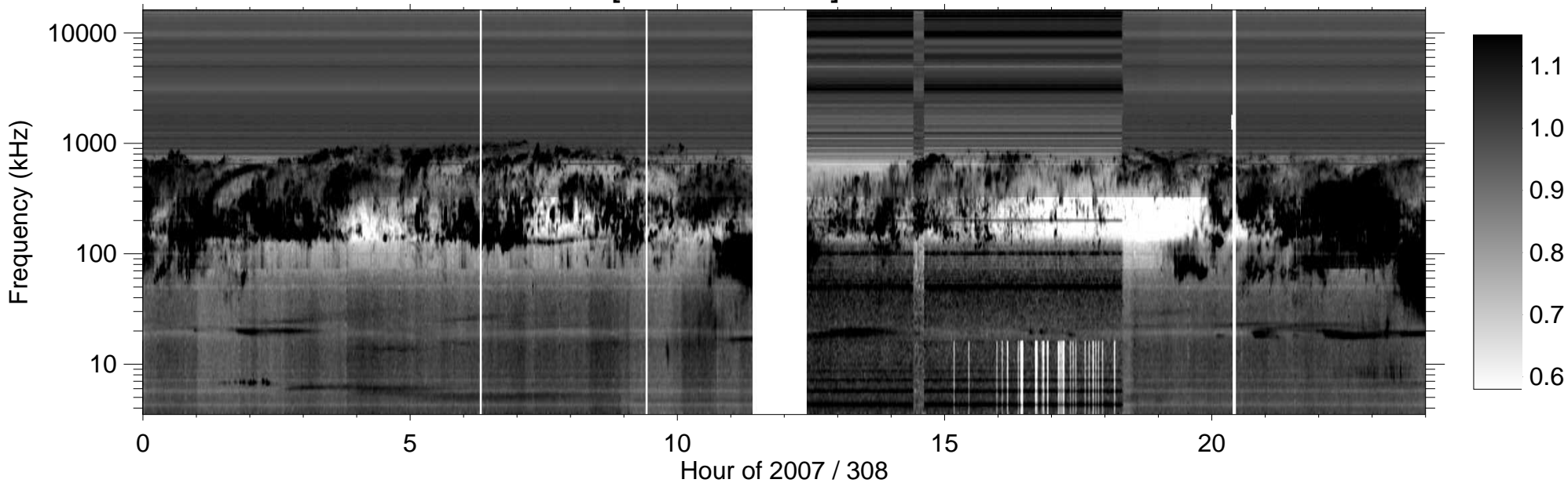
RPWS [ABCH1H2/Ex] (-B) 2007/11/04
