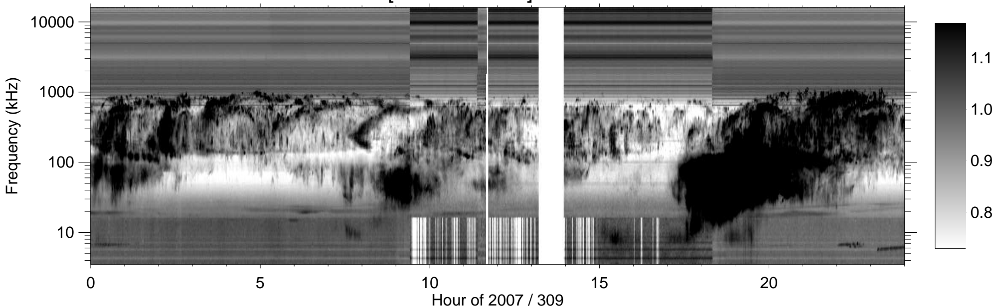
RPWS [ABCH1H2/Ex] (-B) 2007/11/05
