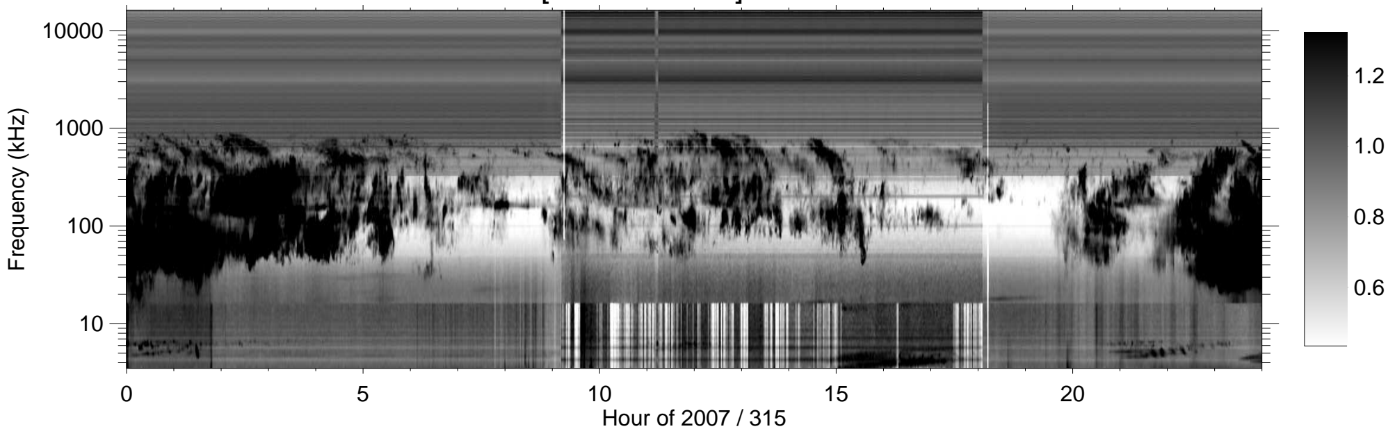
RPWS [ABCH1H2/Ex] (-B) 2007/11/11
