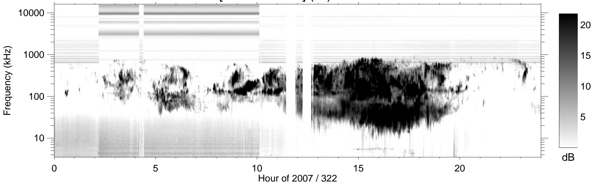
RPWS [ABCH1H2/Ex] (-B) 2007/11/18
