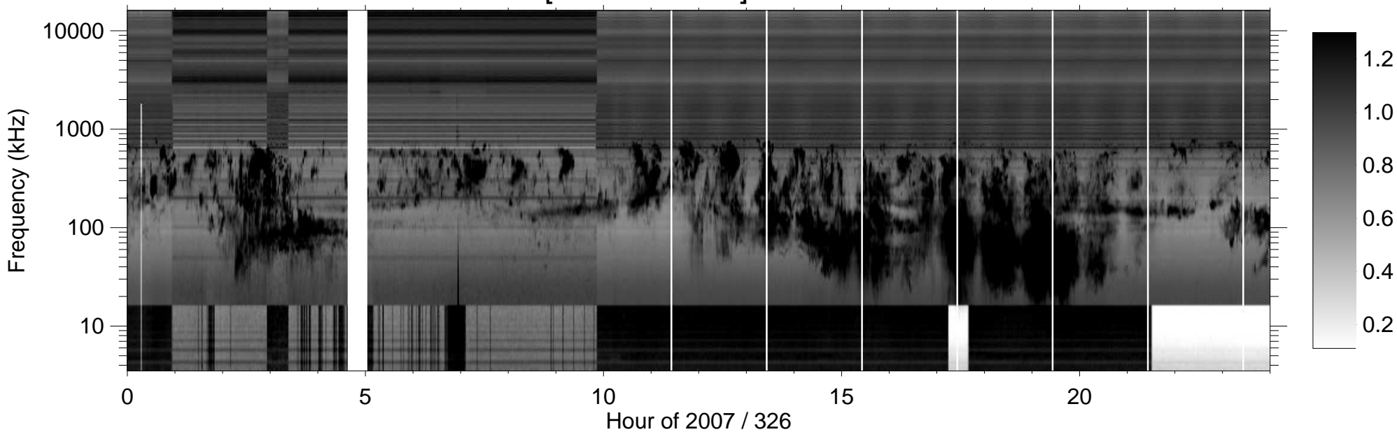
RPWS [ABCH1H2/Ex] (-B) 2007/11/22
