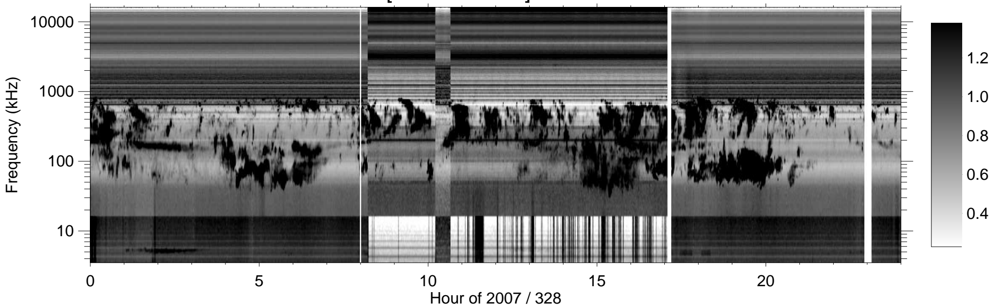
RPWS [ABCH1H2/Ex] (-B) 2007/11/24
