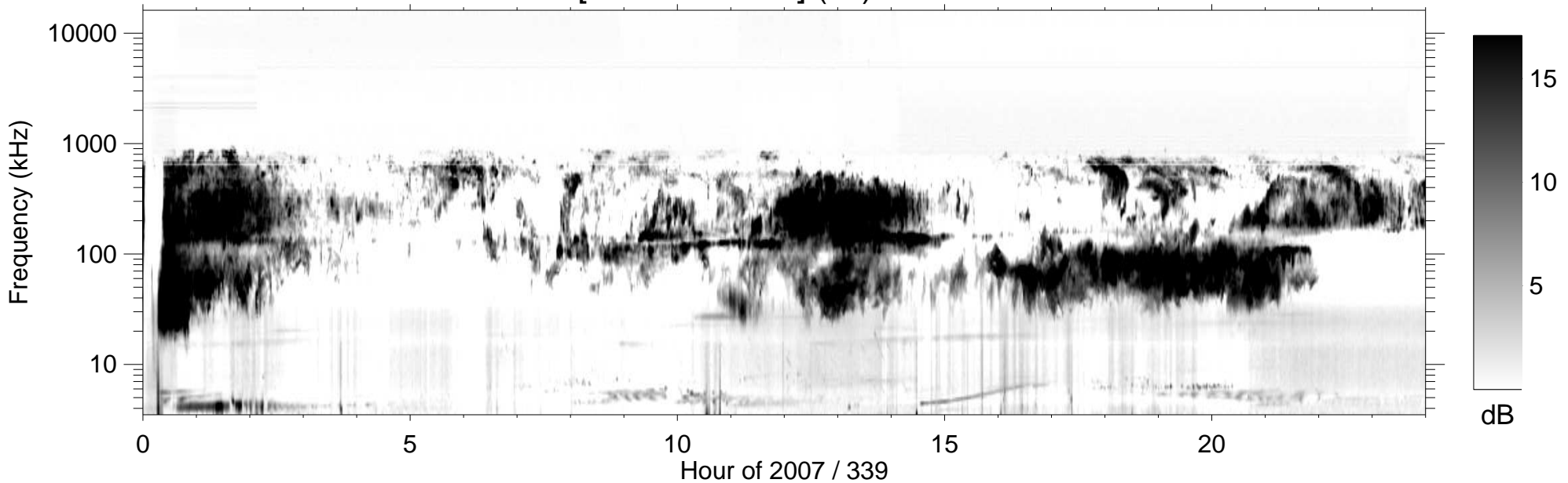
RPWS [ABCH1H2/Ex] (-B) 2007/12/05
