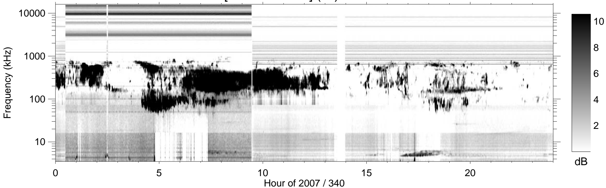
RPWS [ABCH1H2/Ex] (-B) 2007/12/06
