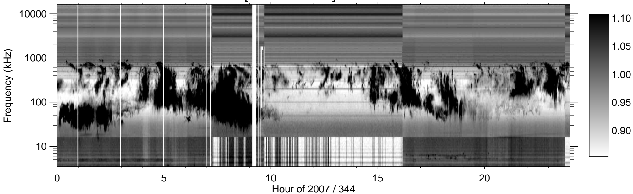
RPWS [ABCH1H2/Ex] (-B) 2007/12/10
