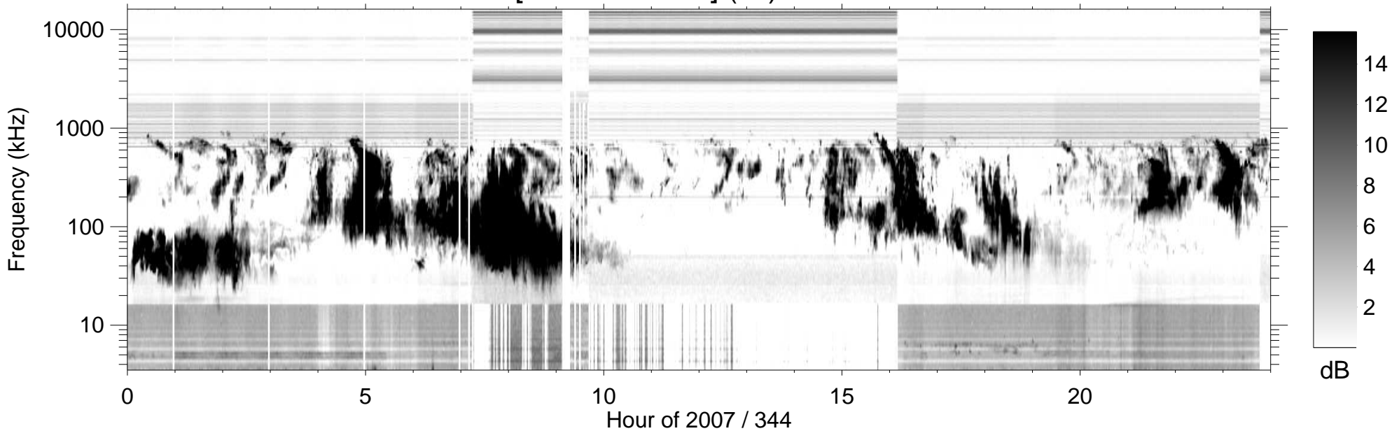
RPWS [ABCH1H2/Ex] (-B) 2007/12/10
