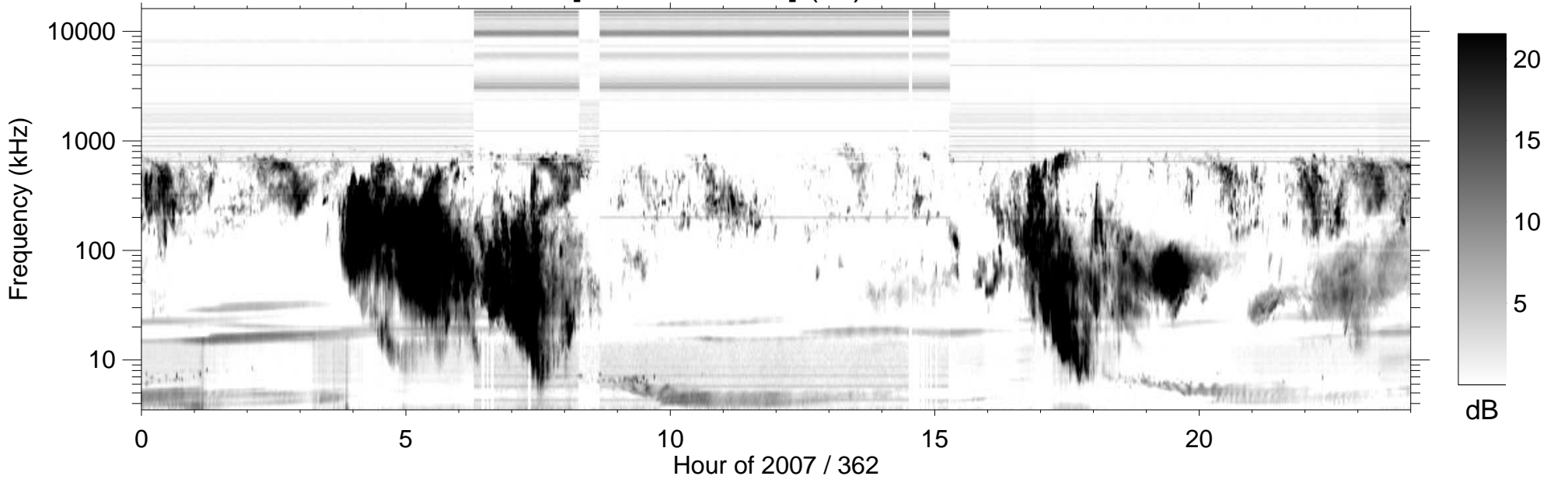
RPWS [ABCH1H2/Ex] (-B) 2007/12/28
