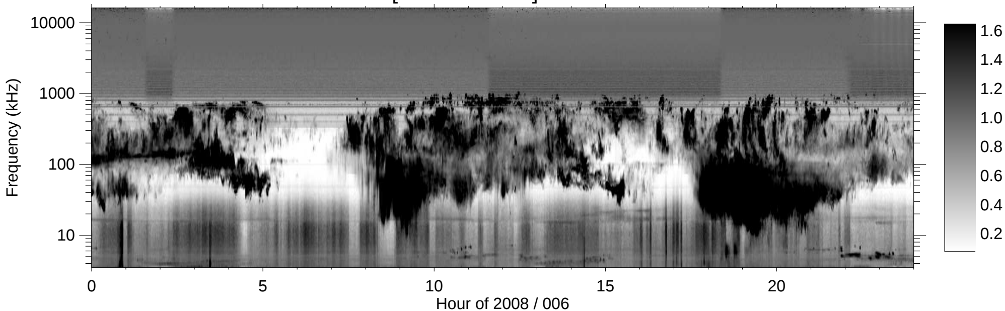
RPWS [ABCH1H2/Ex] (-B) 2008/01/06
