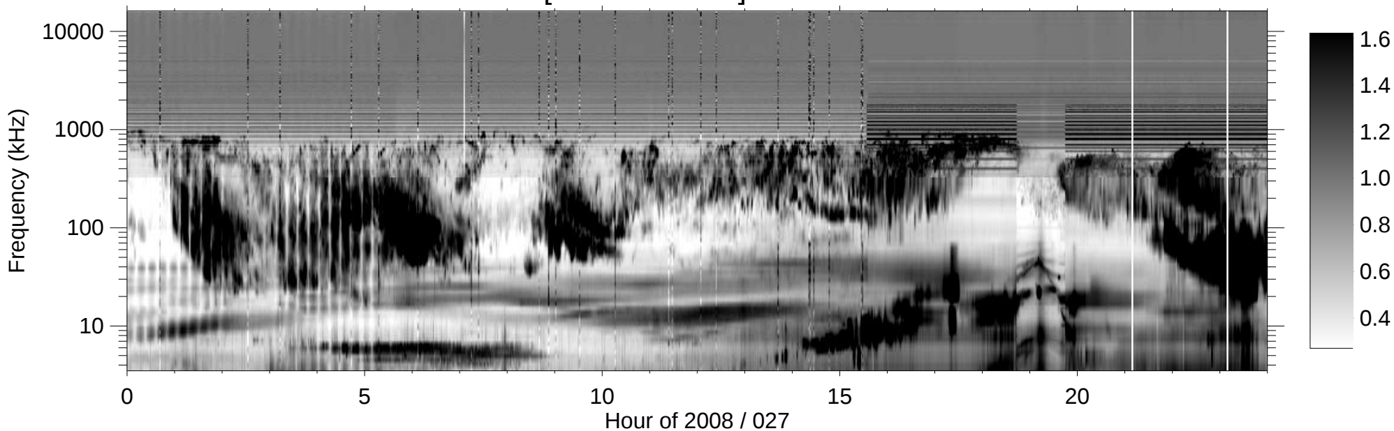
RPWS [ABCH1H2/Ex] (-B) 2008/01/27
