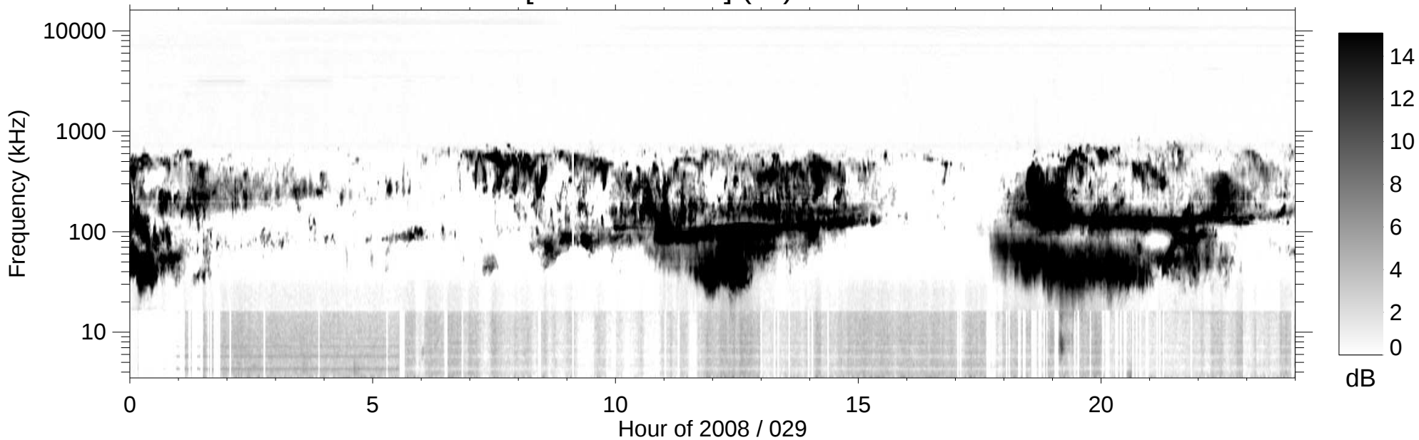
RPWS [ABCH1H2/Ex] (-B) 2008/01/29
