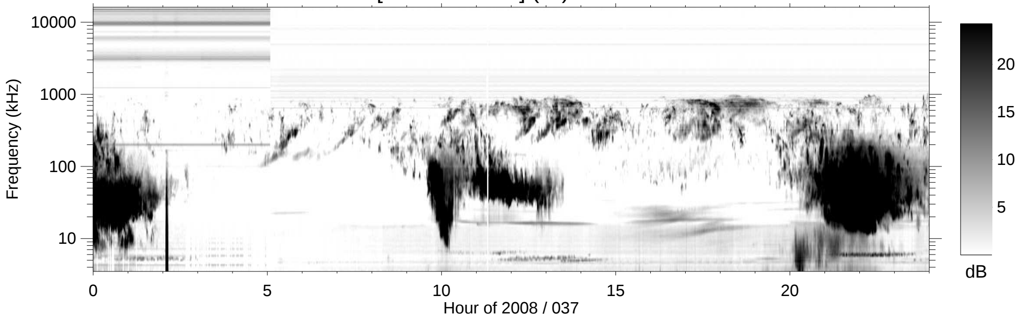
RPWS [ABCH1H2/Ex] (-B) 2008/02/06
