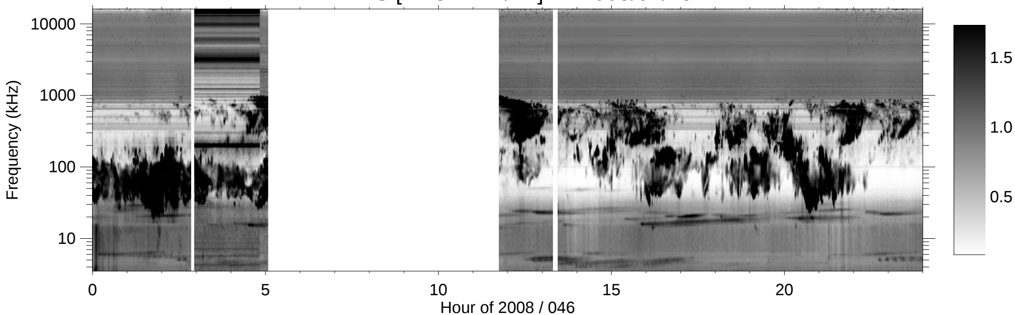
RPWS [ABCH1H2/Ex] (-B) 2008/02/15
