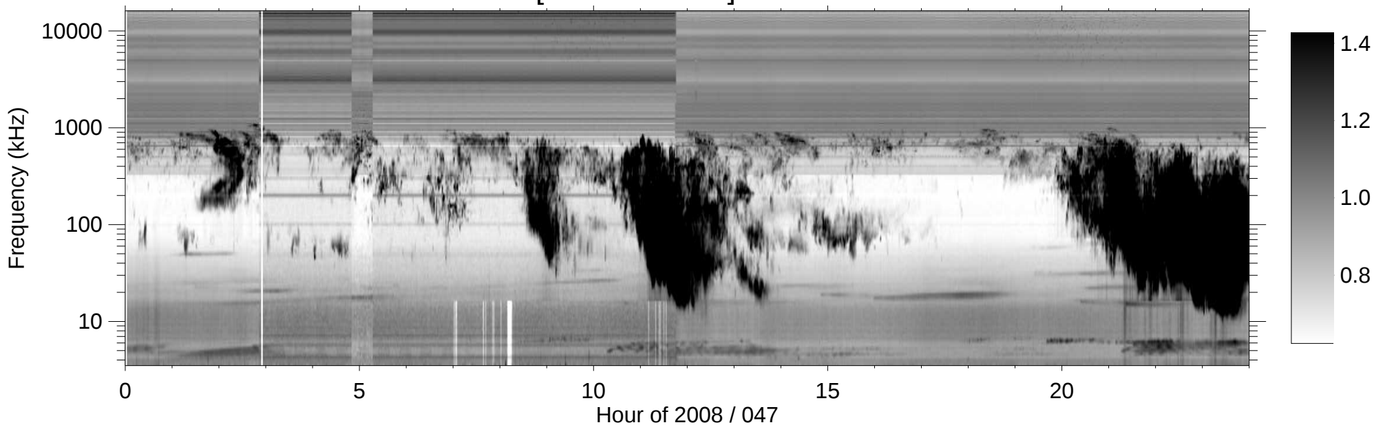
RPWS [ABCH1H2/Ex] (-B) 2008/02/16
