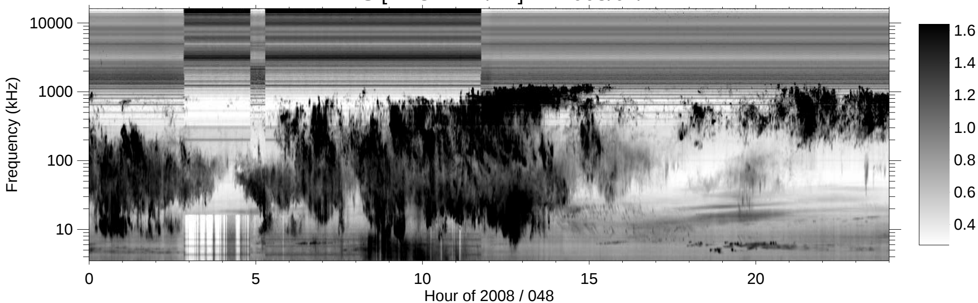
RPWS [ABCH1H2/Ex] (-B) 2008/02/17
