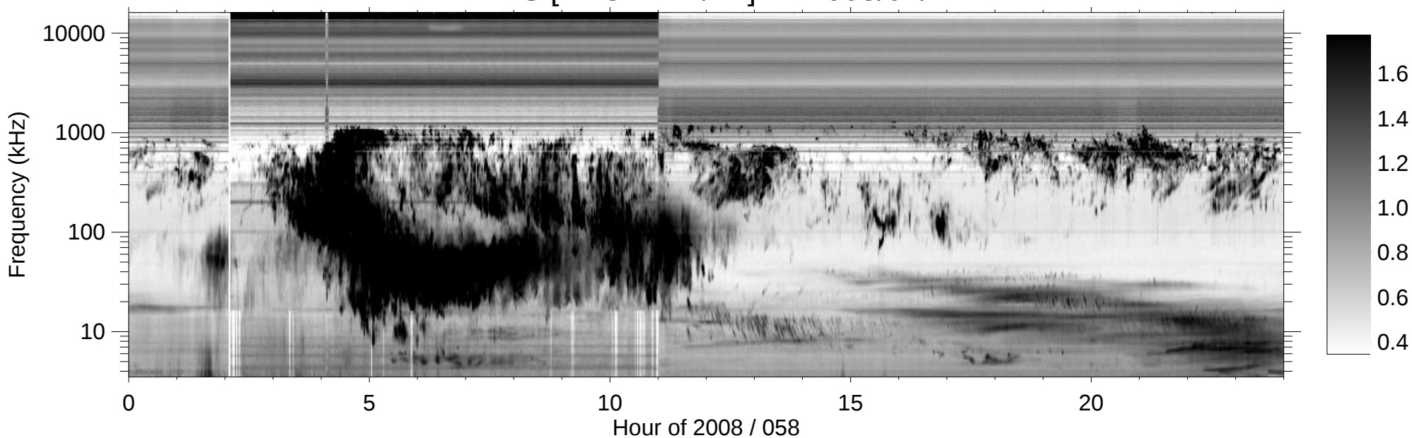
RPWS [ABCH1H2/Ex] (-B) 2008/02/27
