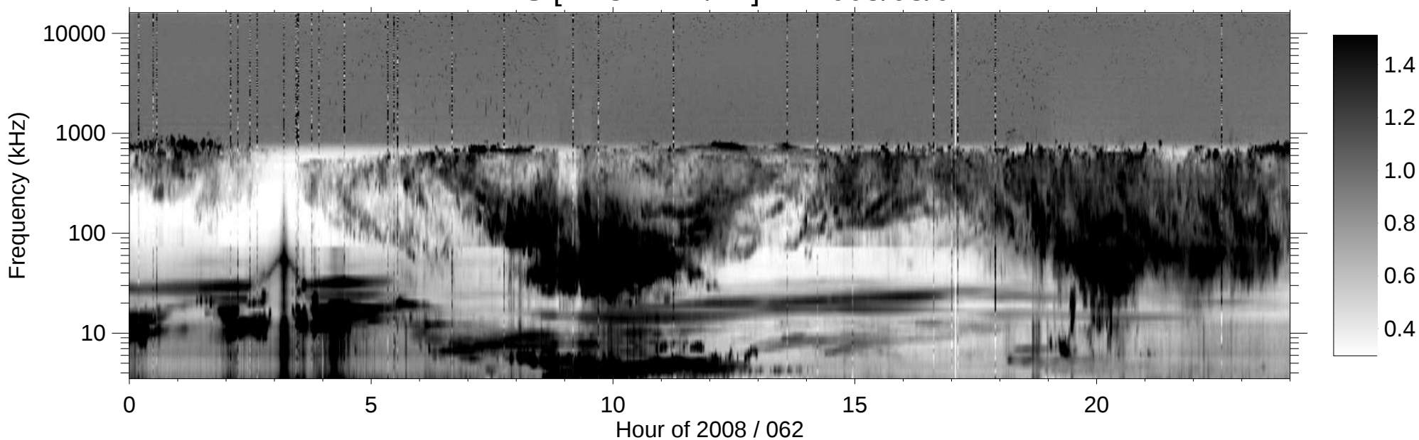
RPWS [ABCH1H2/Ex] (-B) 2008/03/02
