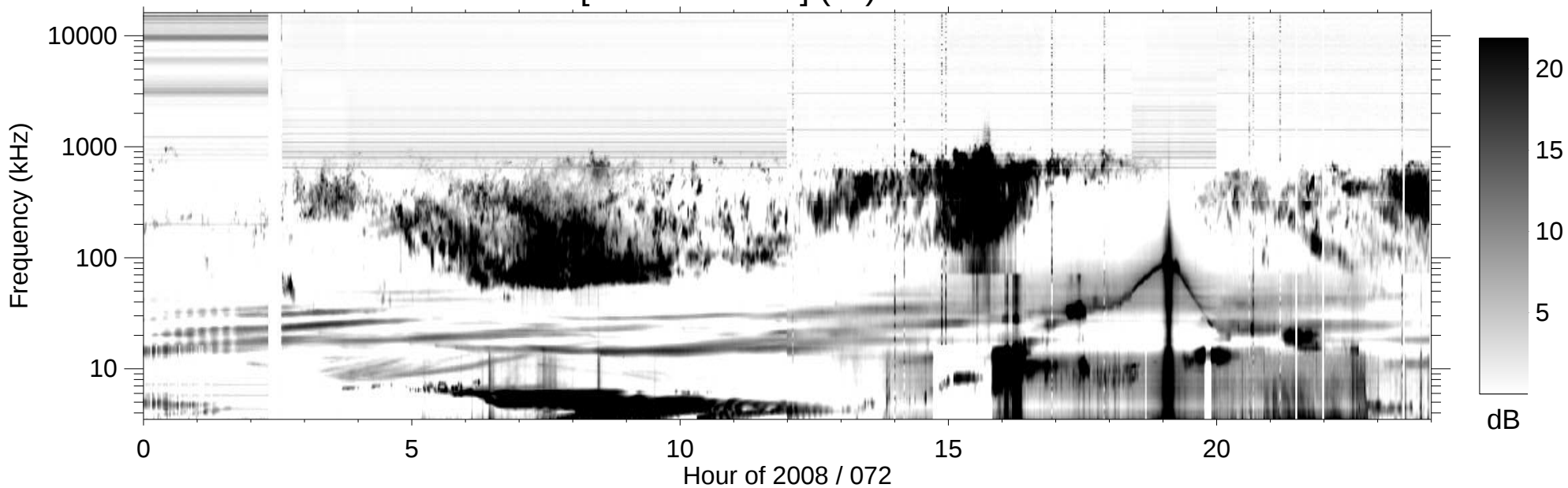
RPWS [ABCH1H2/Ex] (-B) 2008/03/12
