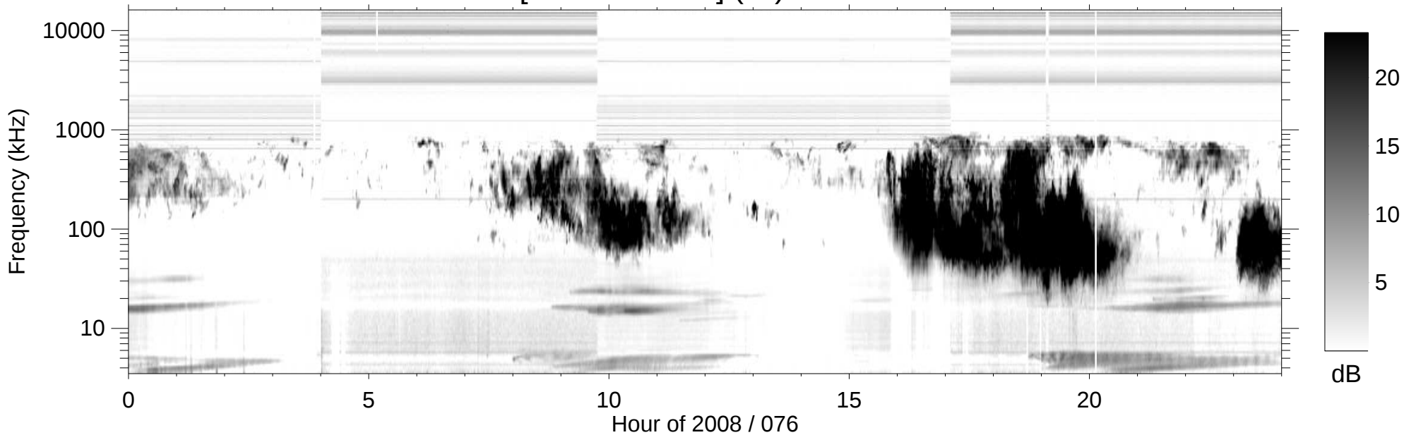
RPWS [ABCH1H2/Ex] (-B) 2008/03/16
