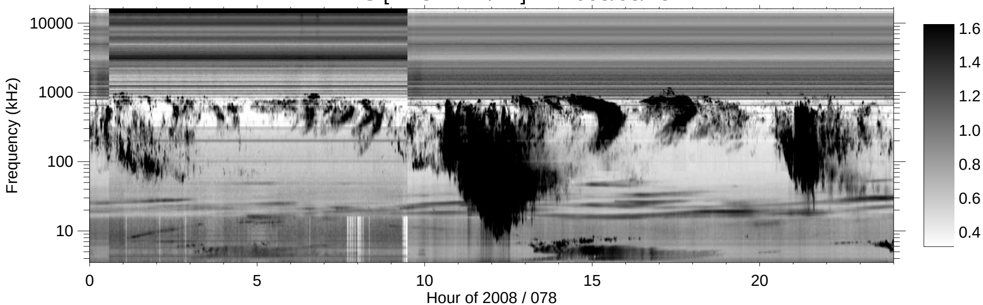
RPWS [ABCH1H2/Ex] (-B) 2008/03/18
