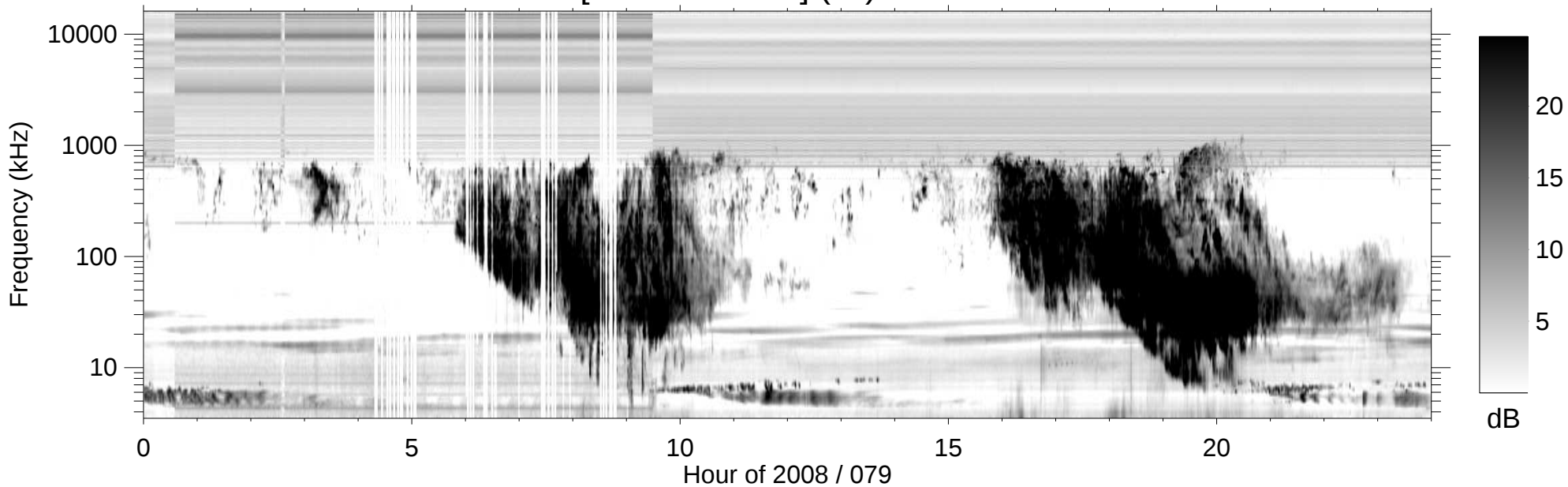
RPWS [ABCH1H2/Ex] (-B) 2008/03/19
