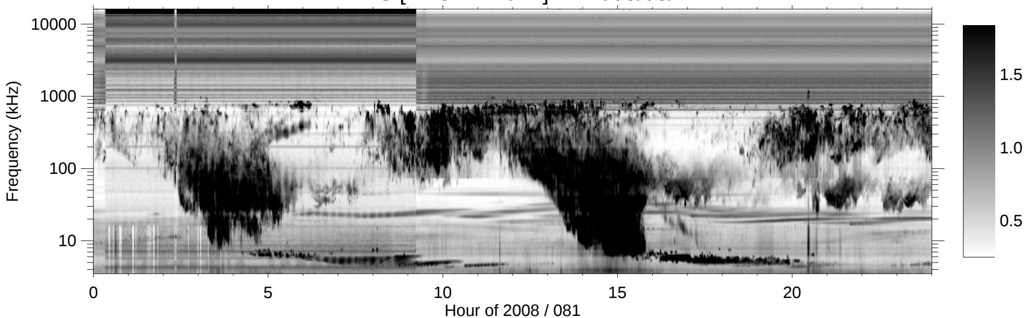
RPWS [ABCH1H2/Ex] (-B) 2008/03/21
