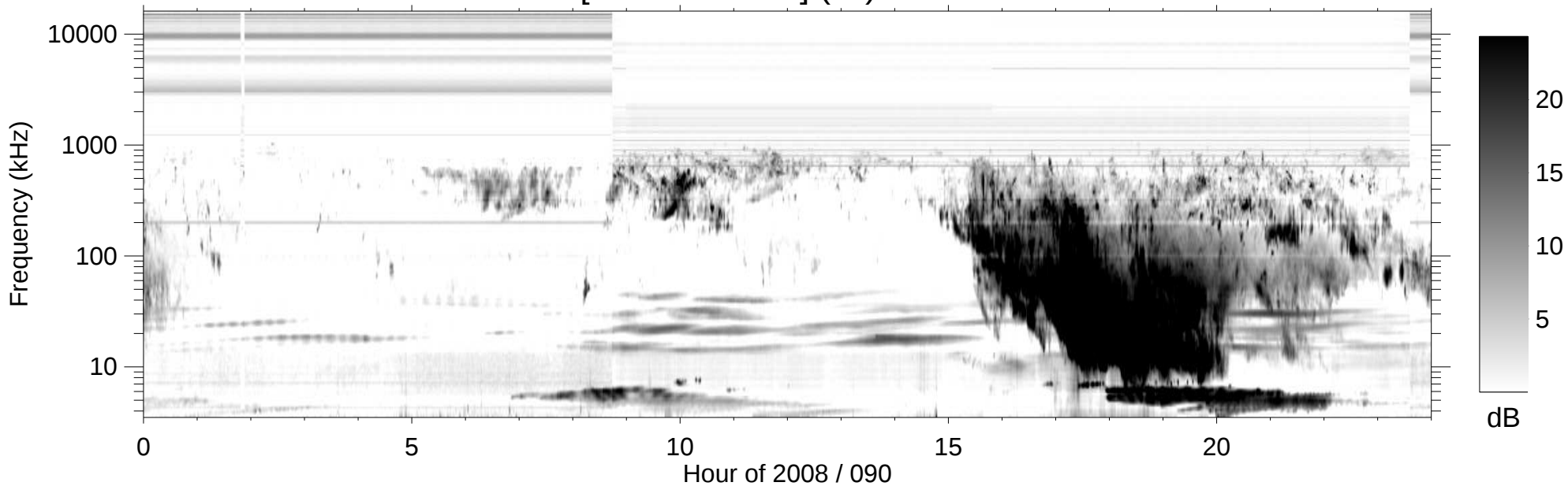
RPWS [ABCH1H2/Ex] (-B) 2008/03/30
