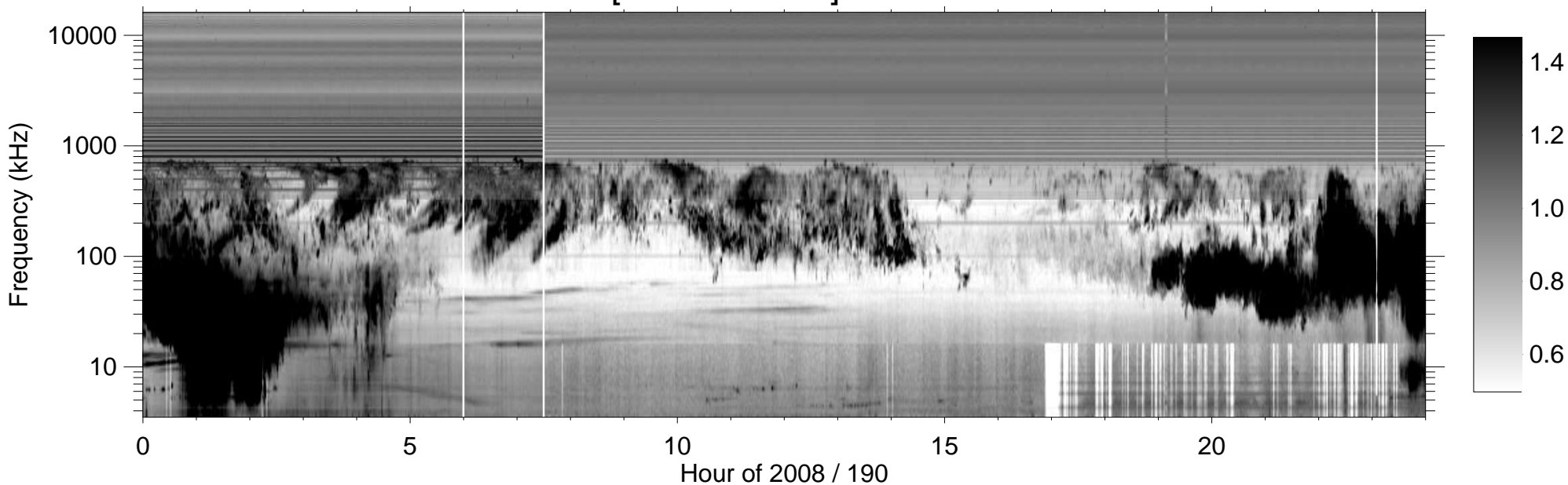
RPWS [ABCH1H2/Ex] (-B) 2008/07/08
