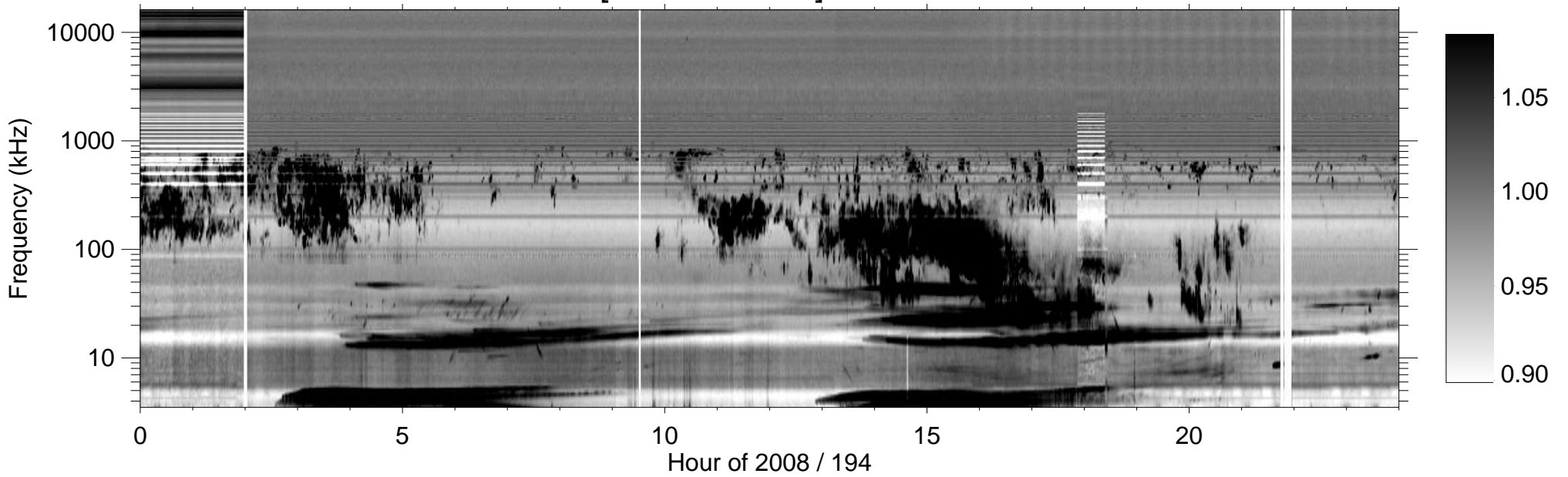
RPWS [ABCH1H2/Ex] (-B) 2008/07/12
