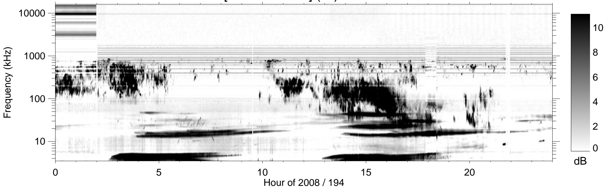
RPWS [ABCH1H2/Ex] (-B) 2008/07/12
