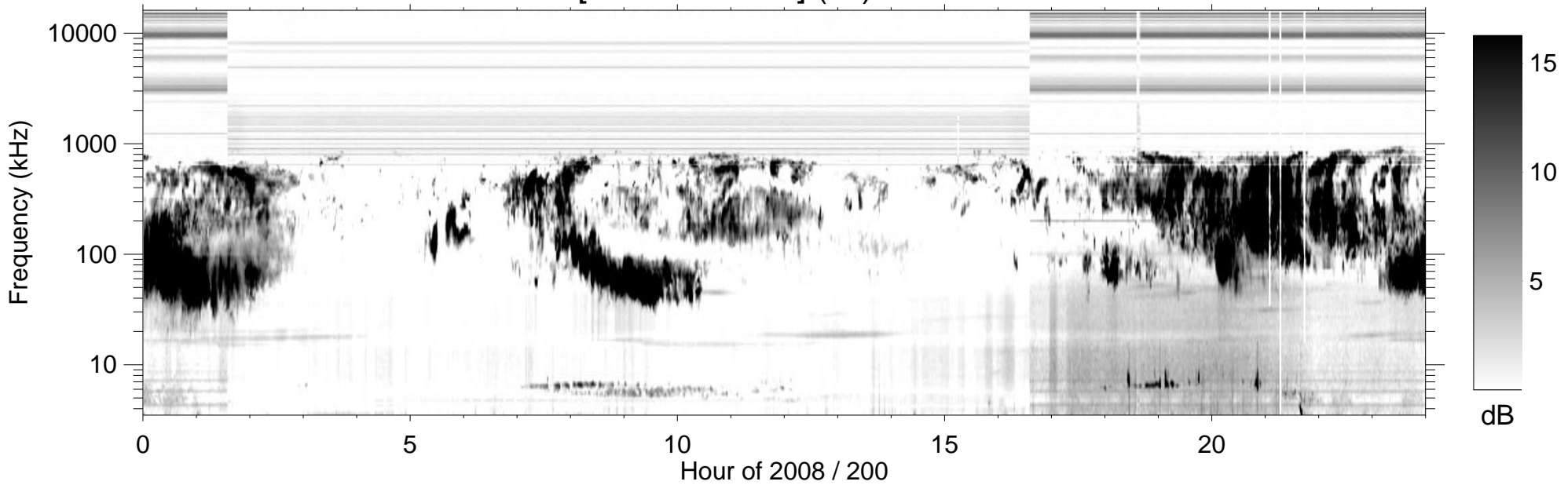
RPWS [ABCH1H2/Ex] (-B) 2008/07/18
