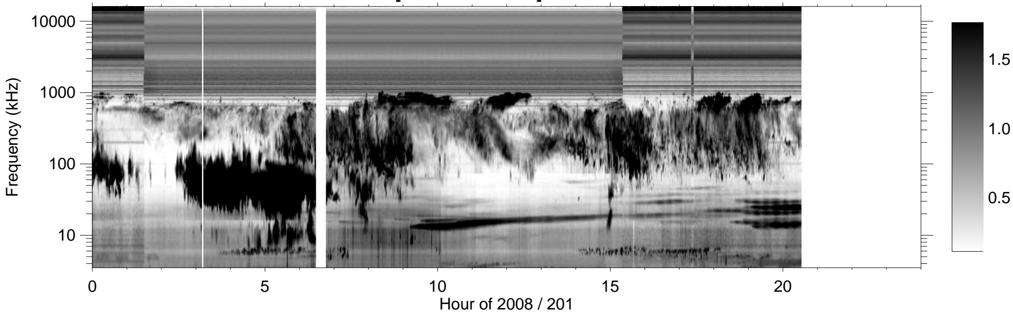
RPWS [ABCH1H2/Ex] (-B) 2008/07/19
