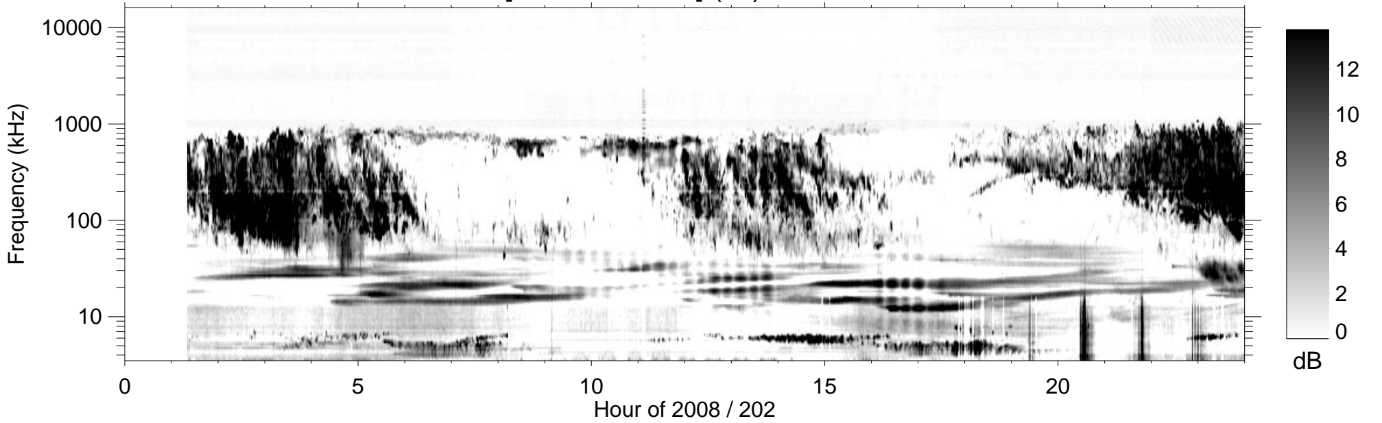
RPWS [ABCH1H2/Ex] (-B) 2008/07/20
