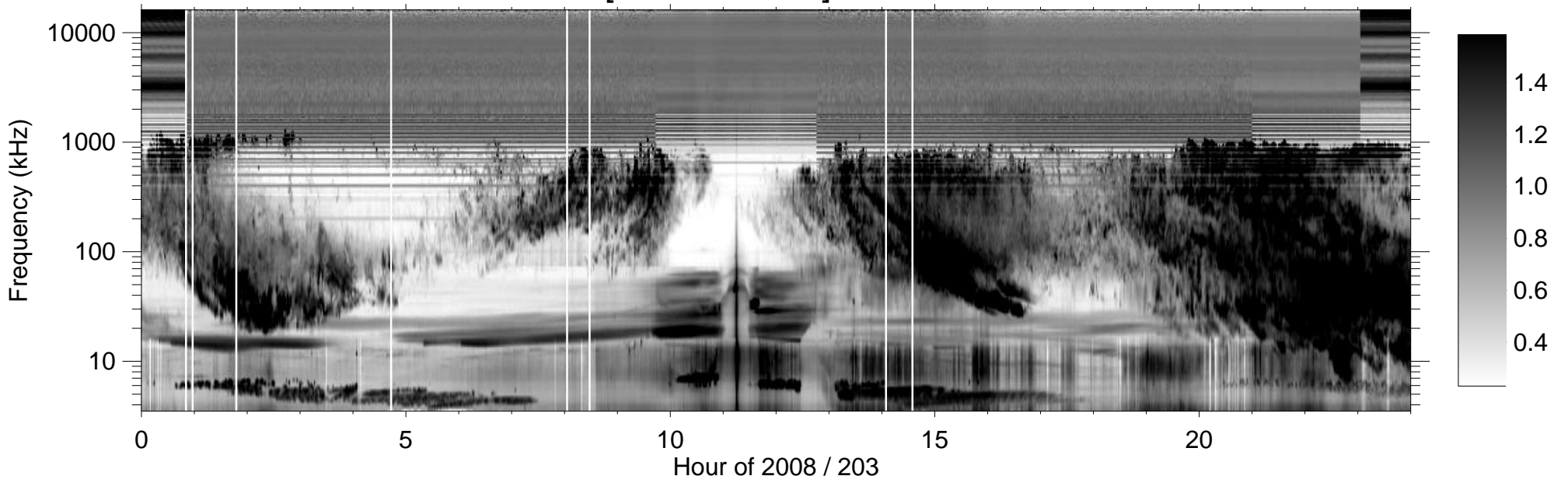
RPWS [ABCH1H2/Ex] (-B) 2008/07/21
