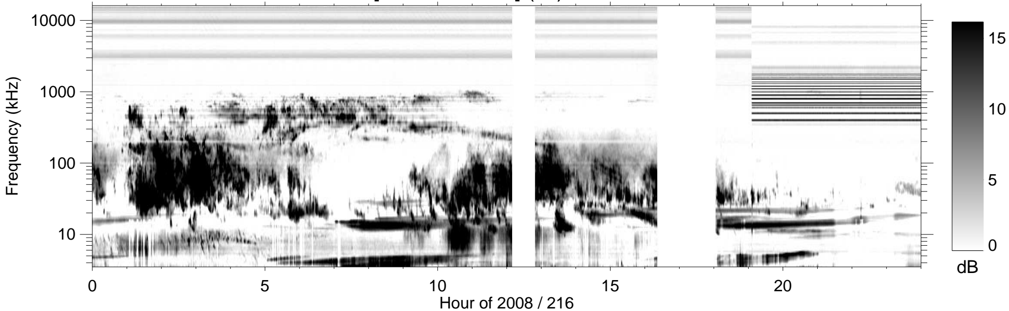
RPWS [ABCH1H2/Ex] (-B) 2008/08/03
