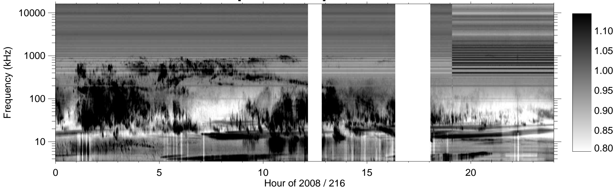
RPWS [ABCH1H2/Ex] (-B) 2008/08/03
